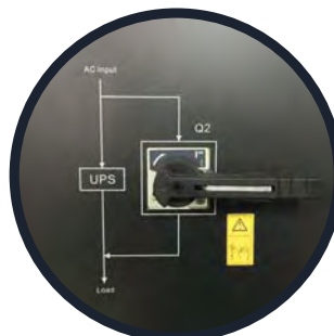
Interruptor Bypass
